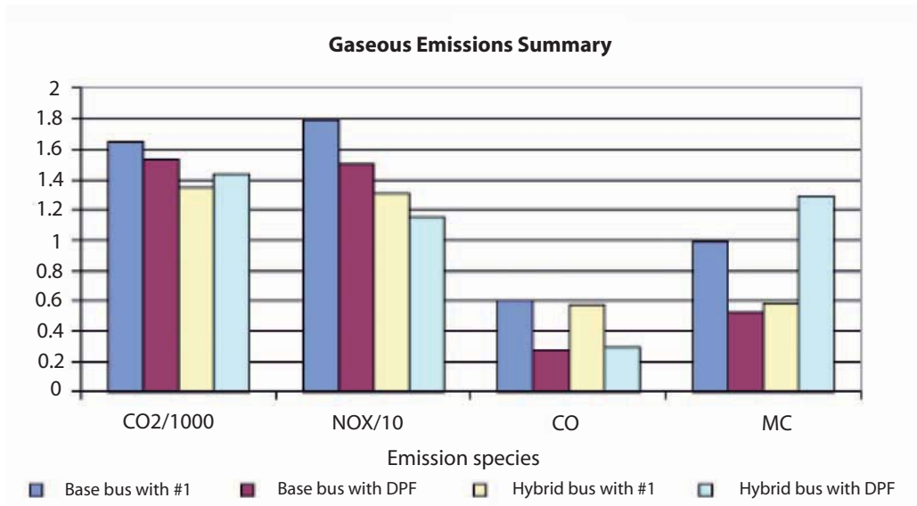
Figure 17 Emissions of buses in NYC, with different engines and fuels
